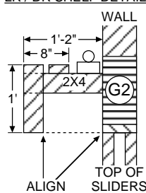
LR / DR SHELF DETAIL
