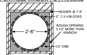
PORTHOLE WINDOW ("G") FRAMING
