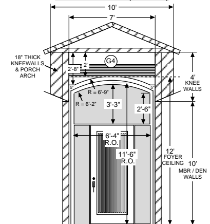
PORCH DETAIL (1/4" = 1')
