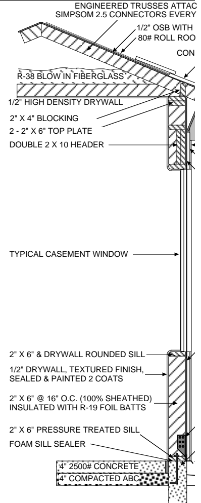
TYPICAL WALL / ROOF CROSS SEC
