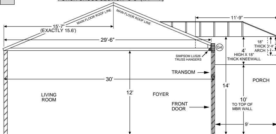
PORCH CROSS SECTION "C-C" (1/4" = 1')
