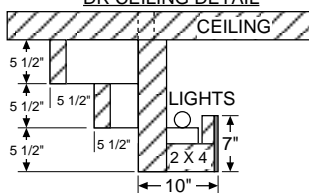
DR CEILING DETAIL
