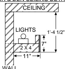
MBR & DEN CEILING DETAIL
